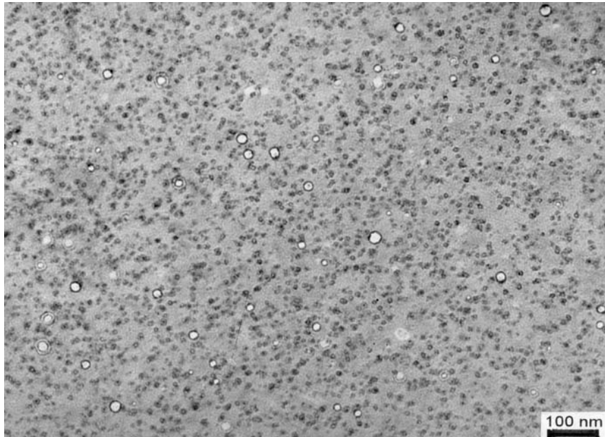
Figure 5. \alpha' -phase precipitates and voids observed in EP-450 irradiated in BN-350 reactor to 56 dpa at 380°C.
