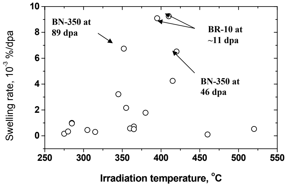
Figure 3. Temperature dependence of the average swelling rate observed in EP-450 with three data points highlighted to show the effect of dpa rate on swelling.
