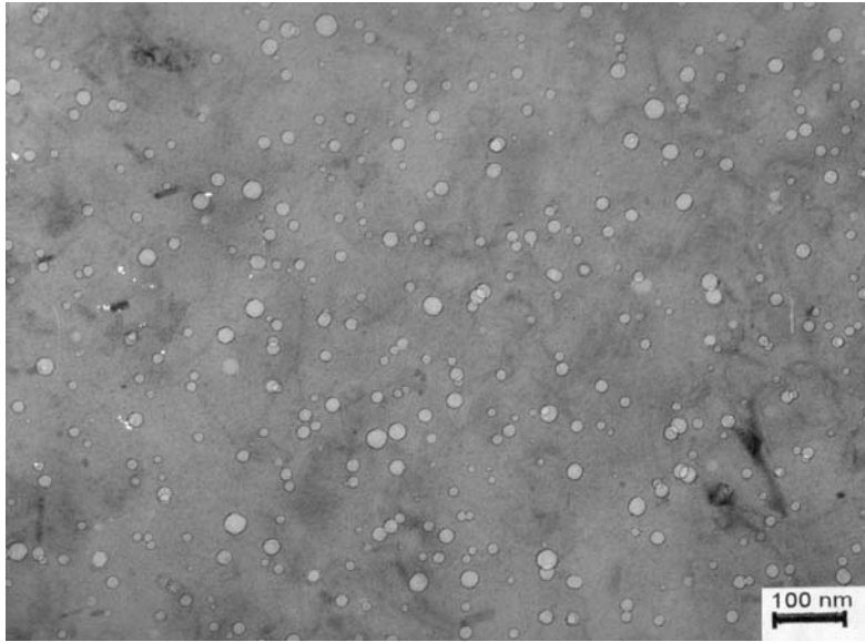
Figure 1. Voids in EP-450 after irradiation in BN-350 to 89 dpa at 352°C.
