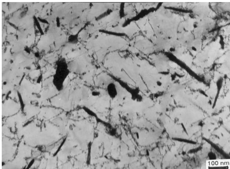
Figure 7. M_2X precipitates observed in EP-450 irradiated in BN-350 reactor to 17 dpa at 690°C.
