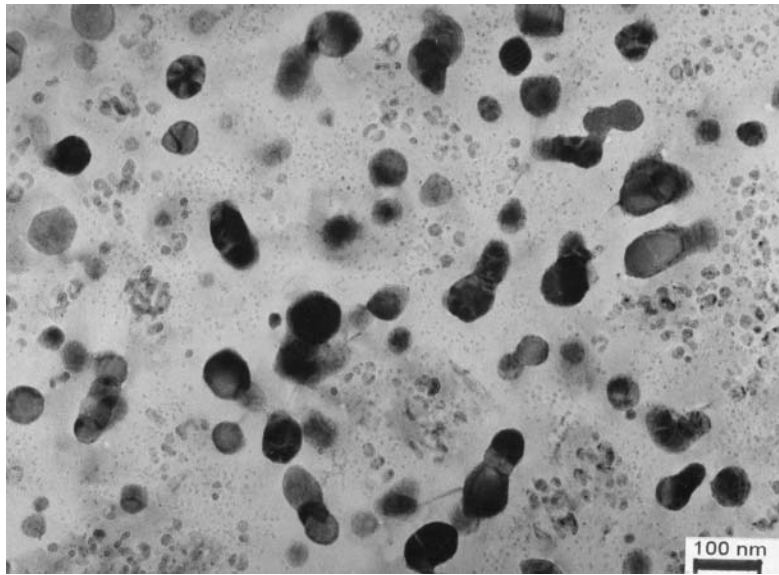
Figure 6. Precipitates of \chi -phase in EP-450 irradiated in BN-600 reactor to 81 dpa at 465°C.
