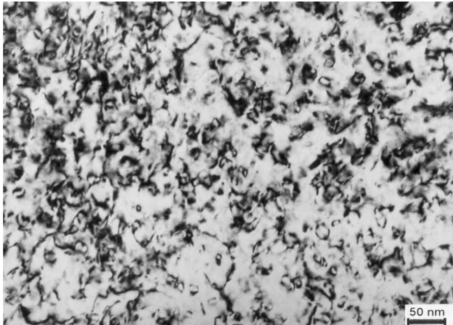
Figure 4. Dislocation structure in ferrite grains of neutron irradiated EP-450 after irradiation in BN-600 to <1 dpa at 360°C.
