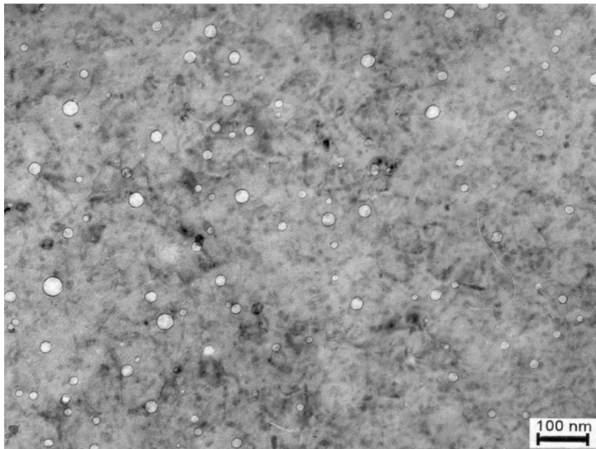
Figure 2. Voids observed in EP-450 after irradiation in BN-350 reactor to 46 dpa at 420°C.
