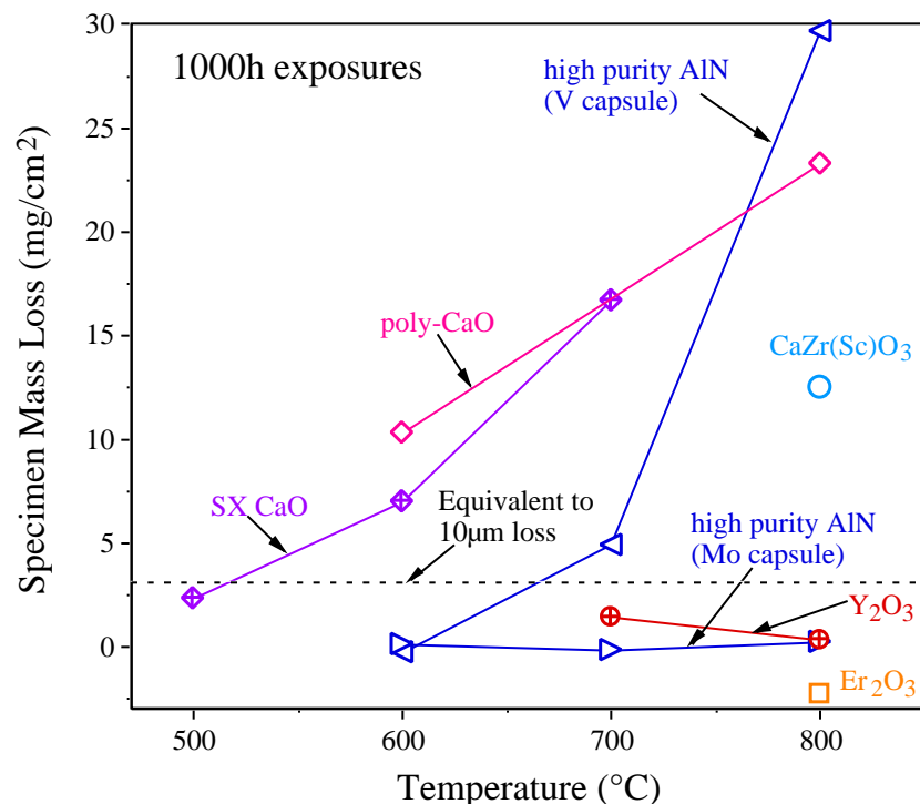
Figure 1. Mass losses for some candidate oxide and nitride materials after 1000h at various temperatures. The results for poly-crystalline and single crystal CaO show severe dissolution above 500°C. The dashed line shows the mass loss associated with the loss of 10µm of coating in a 1000h exposure.
