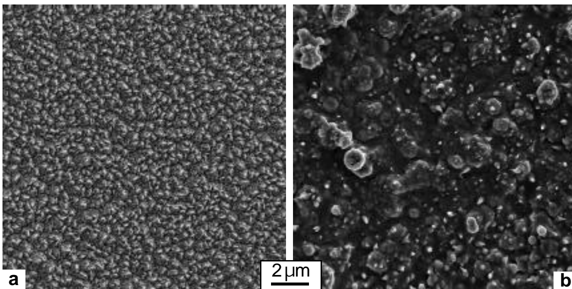
Figure 5. SEM secondary electron plan view images of EB-PVD Y_2O_3 coatings (a) as-received and (b) after exposure to Li at 800^\circ C for 1000h.
