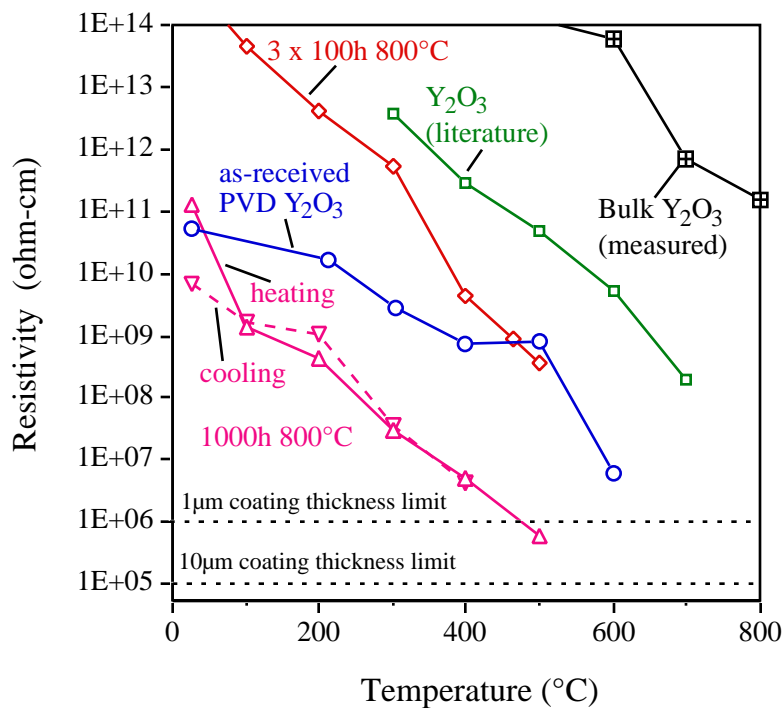
Figure 6. Resistivity as a function of temperature for EB-PVD Y_2O_3 coatings before and after exposure to Li at 800^\circ C . Literature and measured values for bulk Y_2O_3 were much higher.
