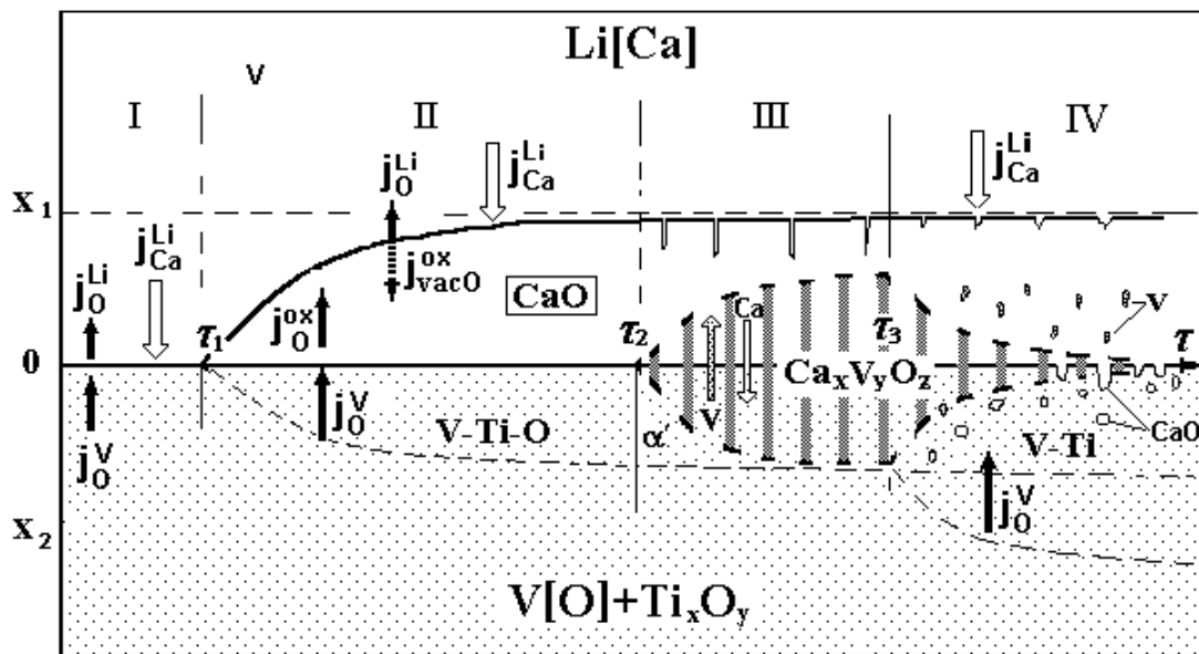
Figure 3. Schematic of the competing processes for the in-situ formation of a CaO layer on a vanadium alloy as a function of time from left to right.[25]
