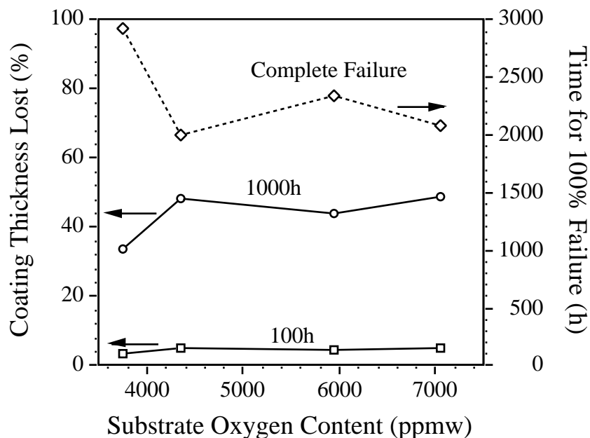
Figure 2. Performance of CaO coatings in Li-2.8at.%Ca at 600°C as a function of oxygen in the V-4Cr-4Ti substrate. Based on the experimentally observed dissolution rate, the percentage of the coating lost with time was calculated as well as the time to complete failure.[18]
