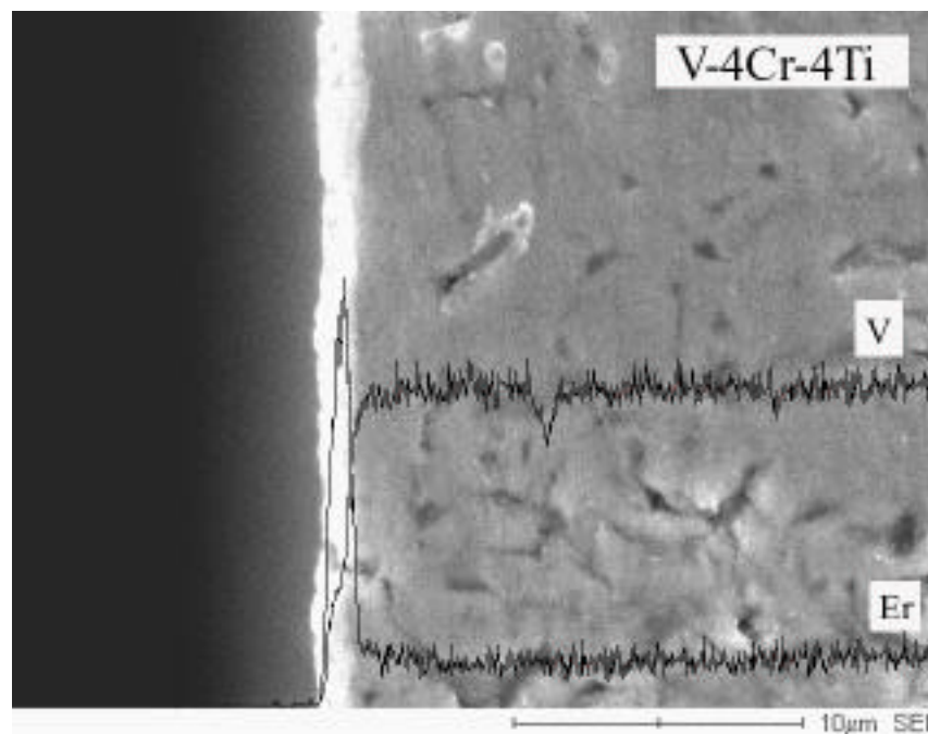
Figure 4. SEM image and EDS line element scan of a cross section of V-4Cr-4Ti oxidized for 6h and annealed for 16h at 700°C, then exposed in Li doped with Er for 300h at 600°C.[26]
